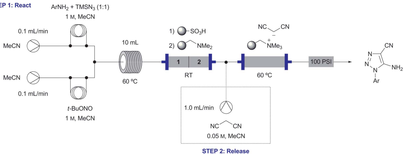
Scheme 3 Flow synthesis of 5-amino-4-cyano-1,2,3-triazoles.
