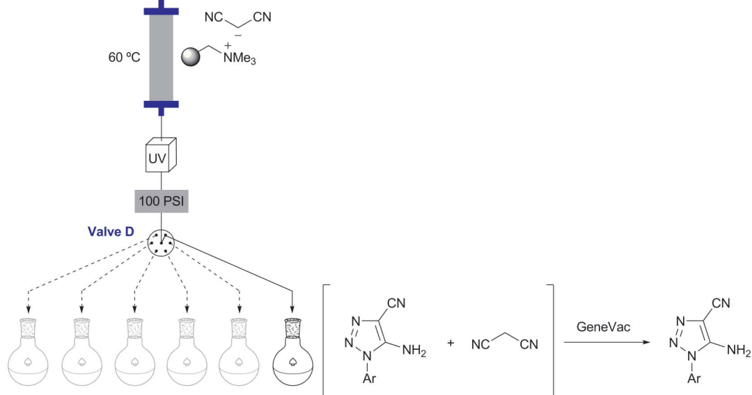
Scheme 4 Automated flow synthesis of 5-amino-4-cyano-1,2,3-triazoles. Step 1: Sample loops A and B are filled by the autosampler, then these starting materials injected and pumped through the system by Pumps A and B to effect azide generation, scavenging and triazole synthesis. Step 2: Sample loop B is filled by the autosampler with a concentrated solution of malononitrile (0.5 M), which is injected, diluted by Pump A and pumped through the system at 0.05 M. Valve A is now in position 2, allowing the wash solution to bypass the CFC and scavenging column to release the desired product from the malononitrile reaction column. Triazole products are collected, then purified by evaporation of malononitrile and MeCN in the GeneVac.
